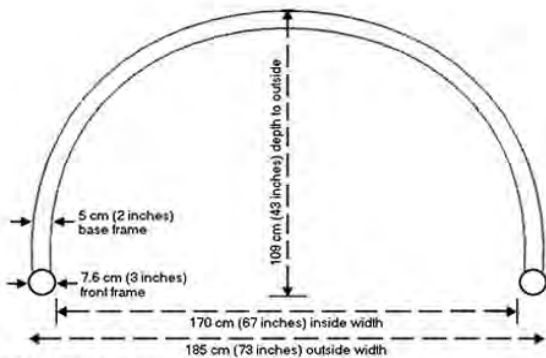
BASE STRUCTURE
