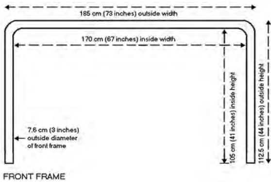
FRONT FRAME
